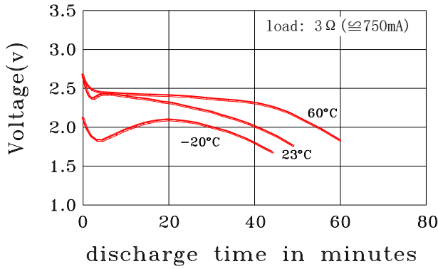
Discharge Characteristics
