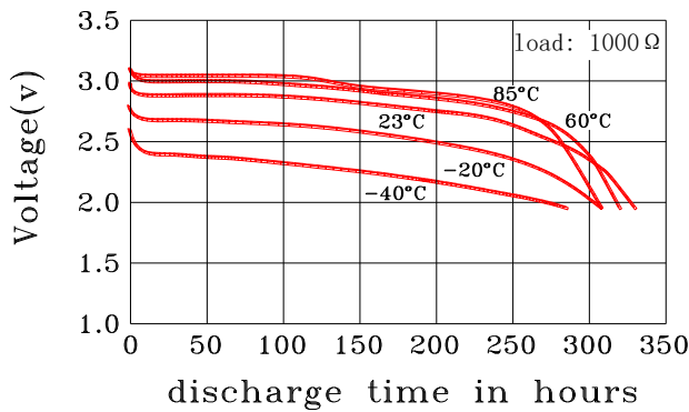
Discharge characteristics on temperature
