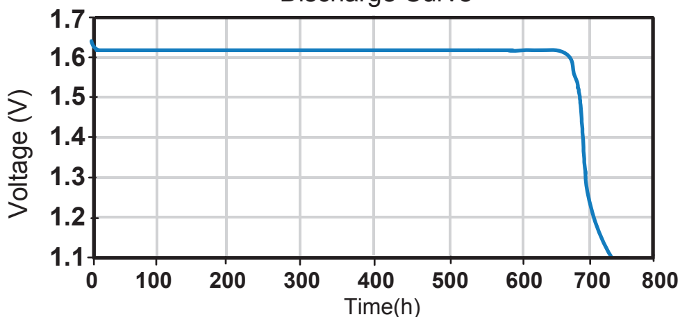
Discharge Curve
