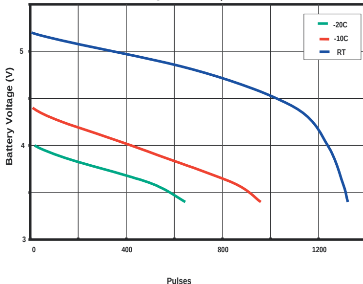
1.2 Amp, 3 sec on/ 7 sec off @ Various Temperatures
