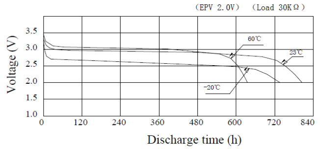
Discharge Characteristics on Temperature
