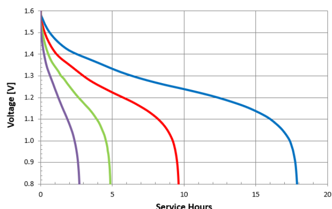
Constant Power
