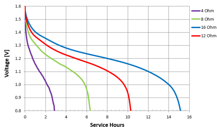
Constant Resistance
