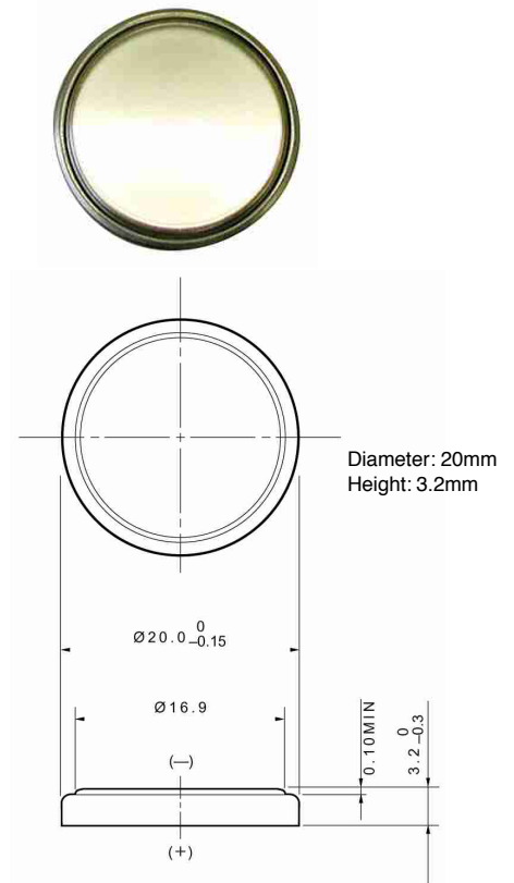
Dimension Drawing
